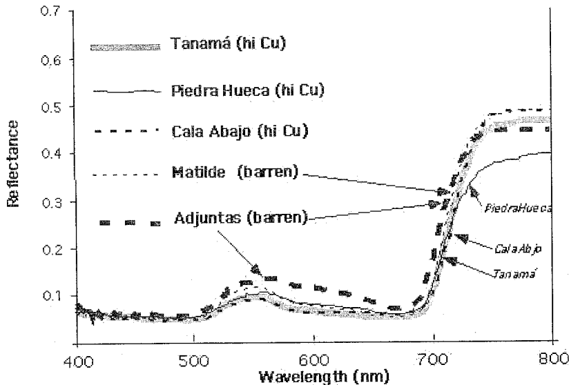
Figure 4. Reflectance of tulipán africano ( Spathodea campanulata ) taken on the Tanamá, Piedra Hueca, and Cala Abajo deposits (all economic deposits), the Matilde stock and barren rocks in Adjuntas. The graph shows that around 550 nm the leaf reflectance of trees on copper bearing substrates is reduced, whereas just above 700 nm, the reflectance shows a shift to the higher wave lengths ('red shift') for leaves of trees on copper bearing substrates.
