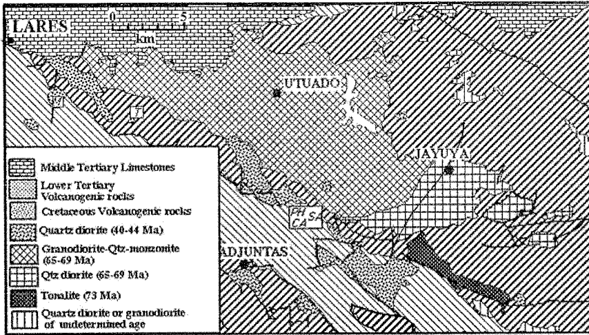
Figure 2. The geology of west central Puerto Rico (based on Barabas, 1982, modified by data from Smith et al. , 1998) with the location of deposits mentioned in the text. M = Matilde stock, T=Tanamá, PH=Piedra Hueca, CA=Cala Abajo, SA=Sapo Alegre.
