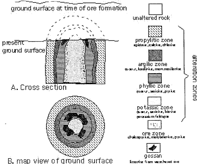
Figure 3. Schematic cross section (A) and map view (B) of a porphyry copper deposit, illustrating that the hydrothermal envelop makes a larger target for exploration (after Lowell and Guilbert, 1970).
